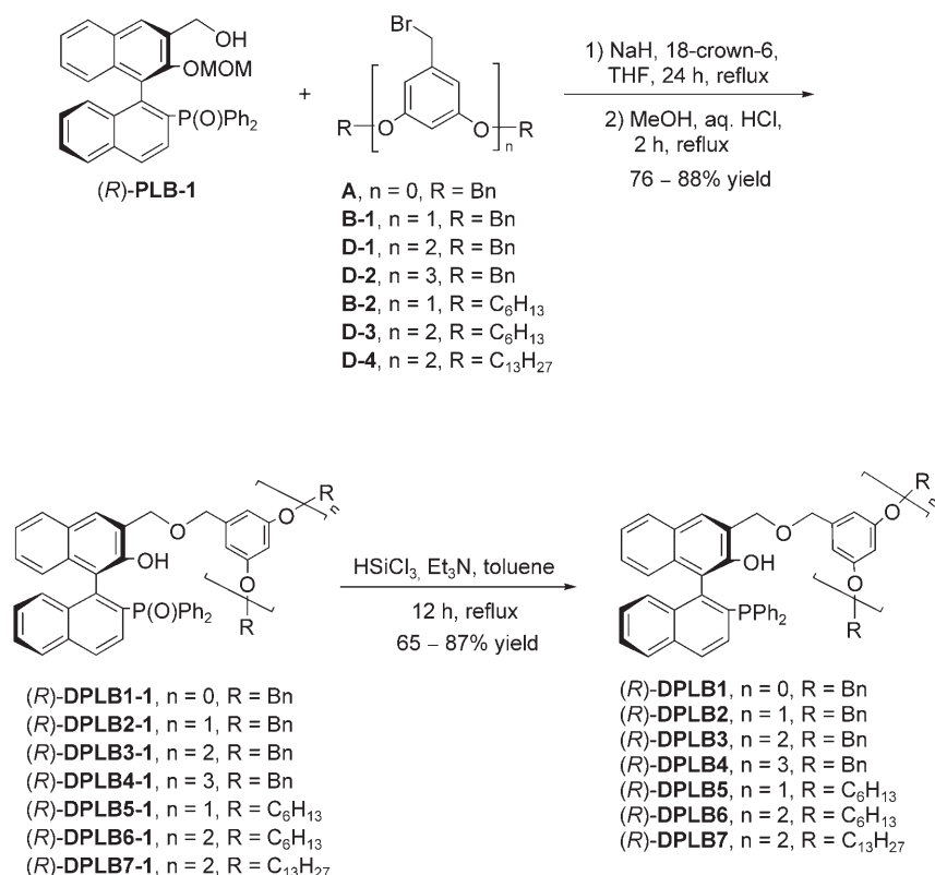
Scheme 1. Synthesis of polyether dendrimer supported chiral Lewis bases ( R )-DPLBs.
